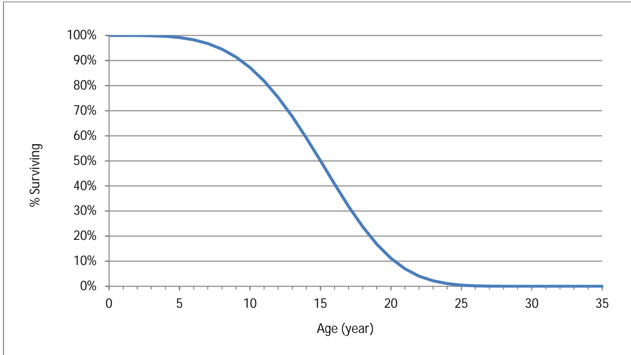
Figure 7: Survival Function for Premium Efficiency Motors 251
