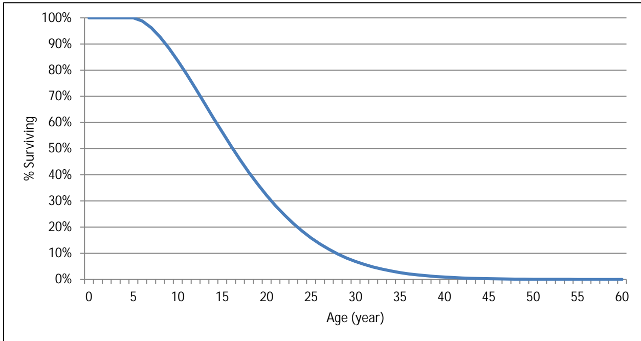
Figure 6: Survival Function for ENERGY STAR® Refrigerators 40
